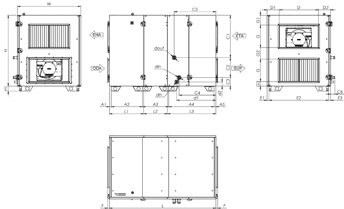
Pav. 8.1.16 AmberAir Compact S-R-3000-H-CO-R-C1 matmenys
