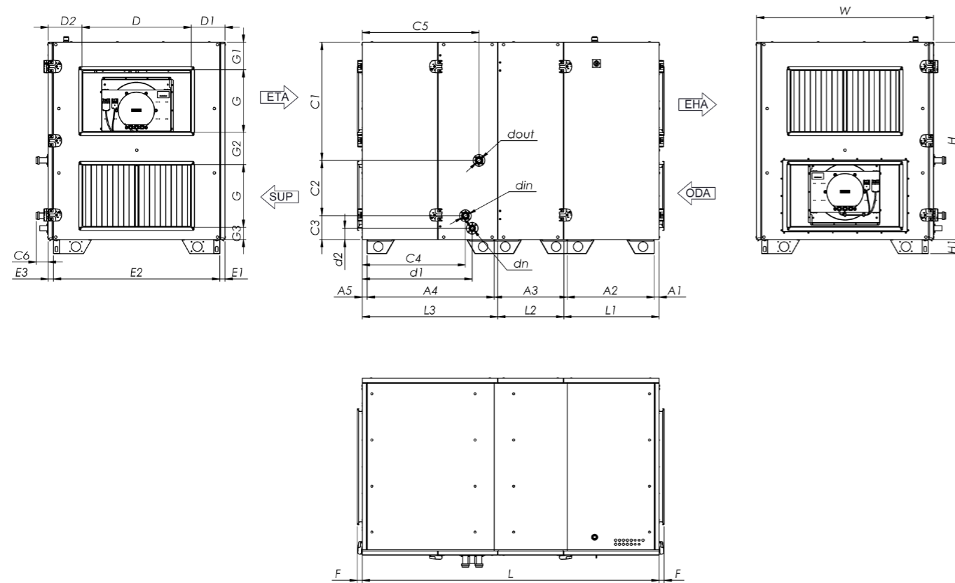
Pav. 8.1.15 AmberAir Compact S-R-3000-H-CO-L-C1 matmenys
