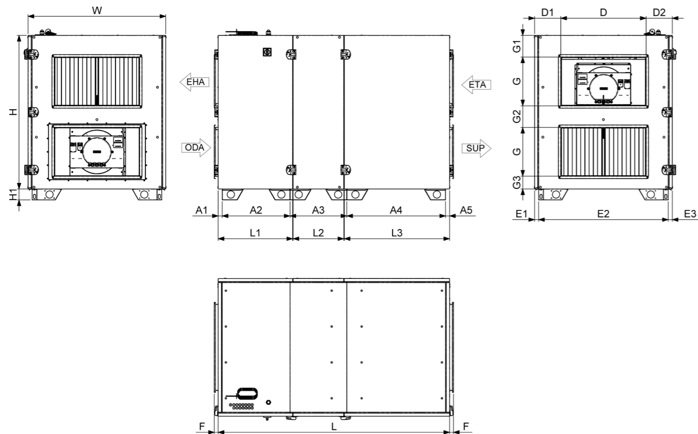
Pav. 8.1.13 AmberAir Compact S-R-3000-H-E-L-C1 matmenys
