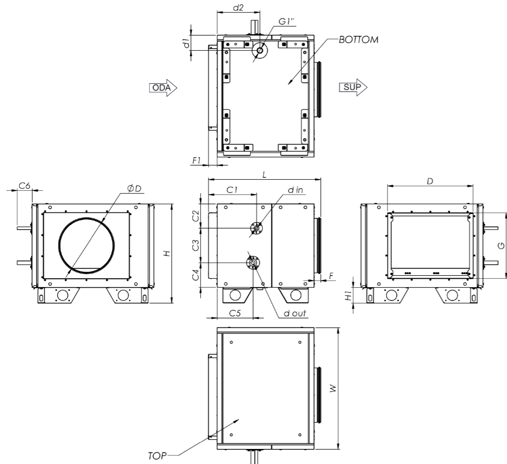
Pav. 8.1.21 Comfort box DX right for AmberAir Compact-S-R-1000-H / AmberAir Compact S-R-1500-H / AmberAir Compact S-R-2000-H matmenys
