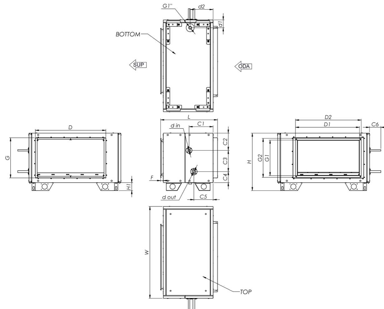
Pav. 8.1.26 Comfort box DX left for AmberAir Compact S-R-3000-H matmenys
