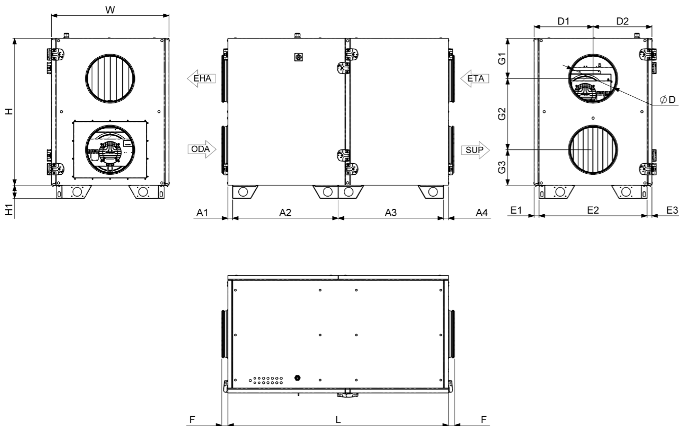
Pav. 8.1.2 AmberAir Compact S-R-1000-H-E-R-C1 / AmberAir Compact S-R-1500-H-E-R-C1 matmenys
