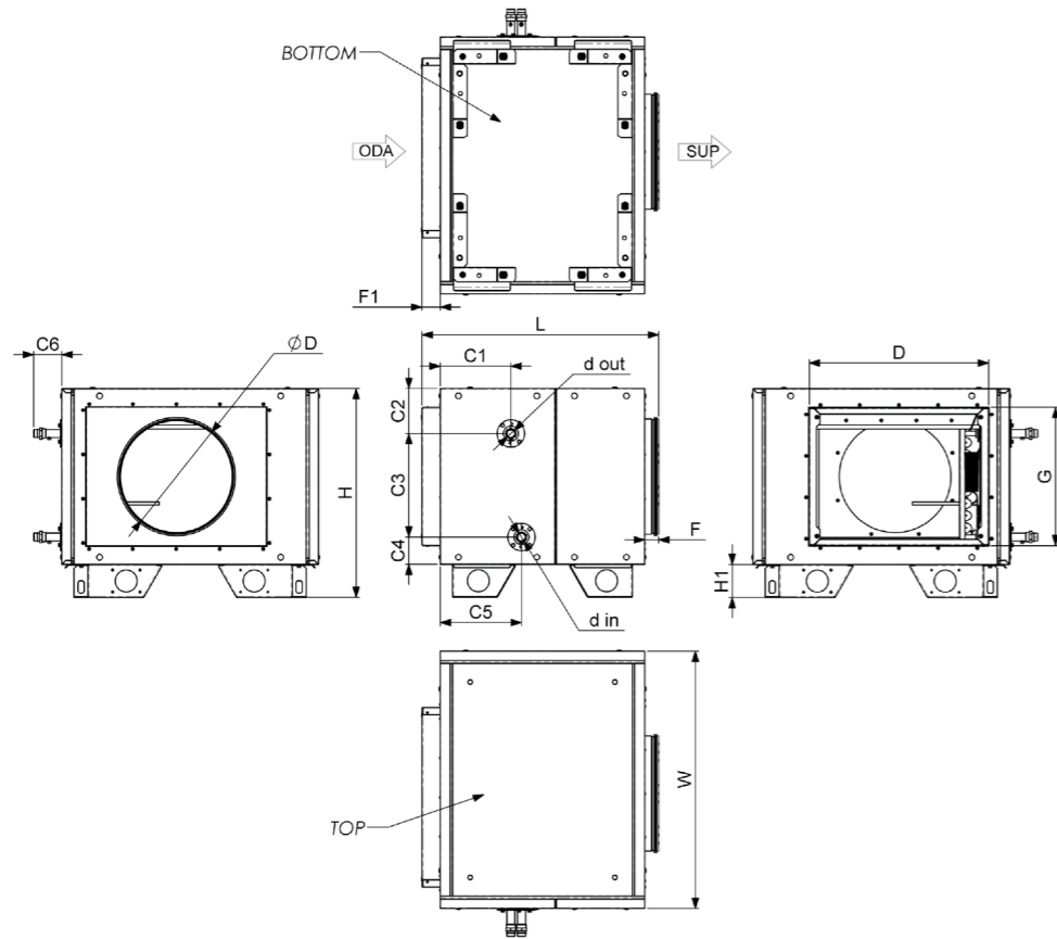
Pav. 8.1.19 Comfort box WH right for AmberAir Compact-S-R-1000-H / AmberAir Compact S-R-1500-H / AmberAir Compact S-R-2000-H matmenys
