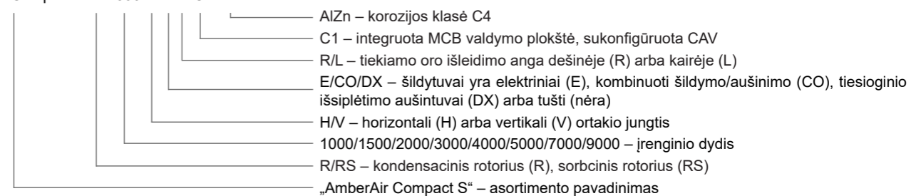
AmberAir Compact S-R-1500-H-E-R-C1 AlZn
