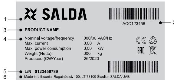
Figure 1.1 - Technical label
