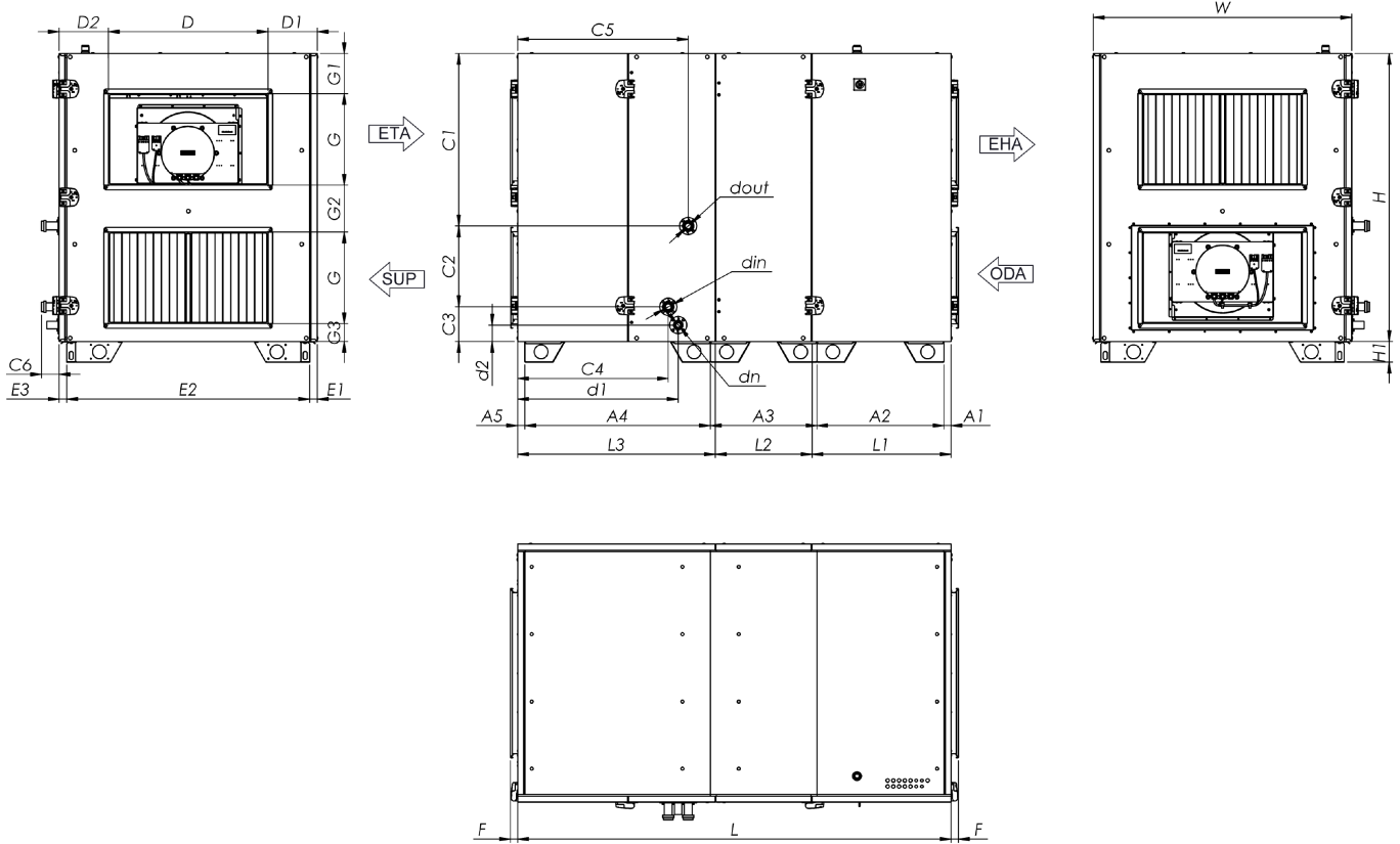
Fig. 8.1.15 Wymiary AmberAir Compact S-R-3000-H-CO-L-C1 / AmberAir Compact S-R-4000-H-CO-L-C1 / AmberAir Compact S-R-5000-H-CO-L-C1
