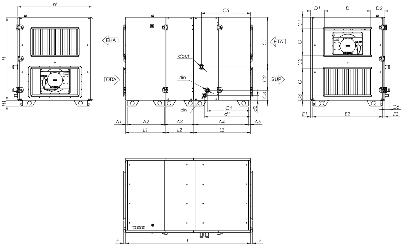
Fig. 8.1.16 Wymiary AmberAir Compact S-R-3000-H-CO-R-C1 / AmberAir Compact S-R-4000-H-CO-R-C1 / AmberAir Compact S-R-5000-H-CO-R-C1
