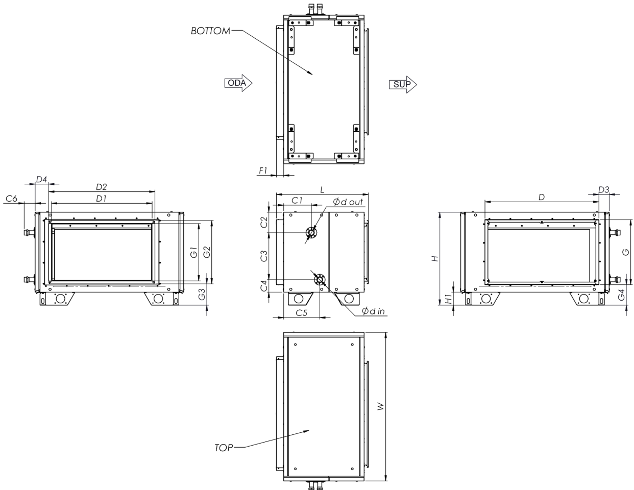
Fig. 8.1.28 Wymiary Comfort box WH right for AmberAir Compact S-R-3000-H / AmberAir Compact S-R-4000-H / AmberAir Compact S-R-5000-H / AmberAir Compact S-R-7000-H / AmberAir Compact S-R-9000-H
