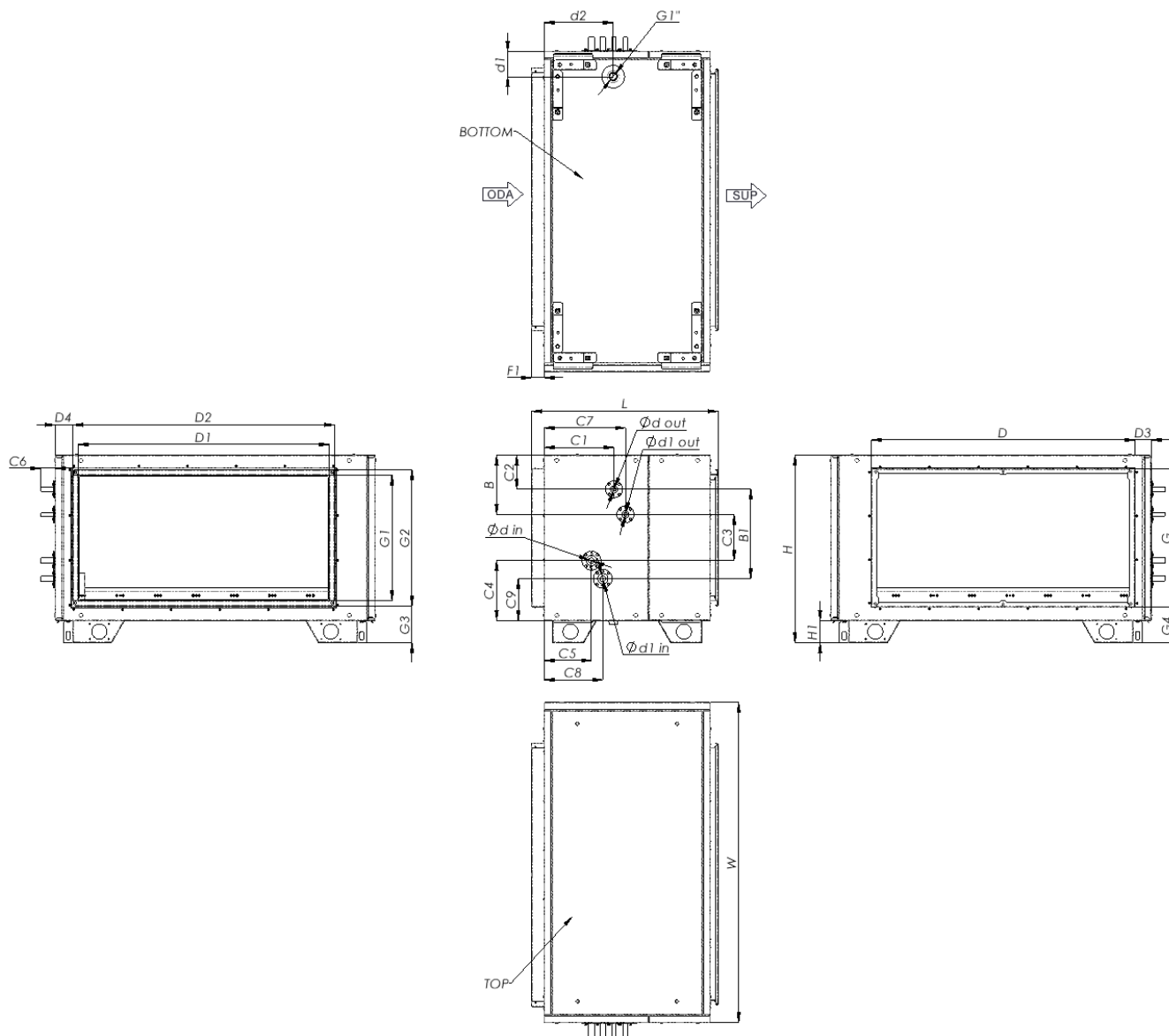
Fig. 8.1.31 Wymiary Comfort box DX right for AmberAir Compact S-R-5000-H / AmberAir Compact S-R-7000-H / AmberAir Compact S-R-9000-H
