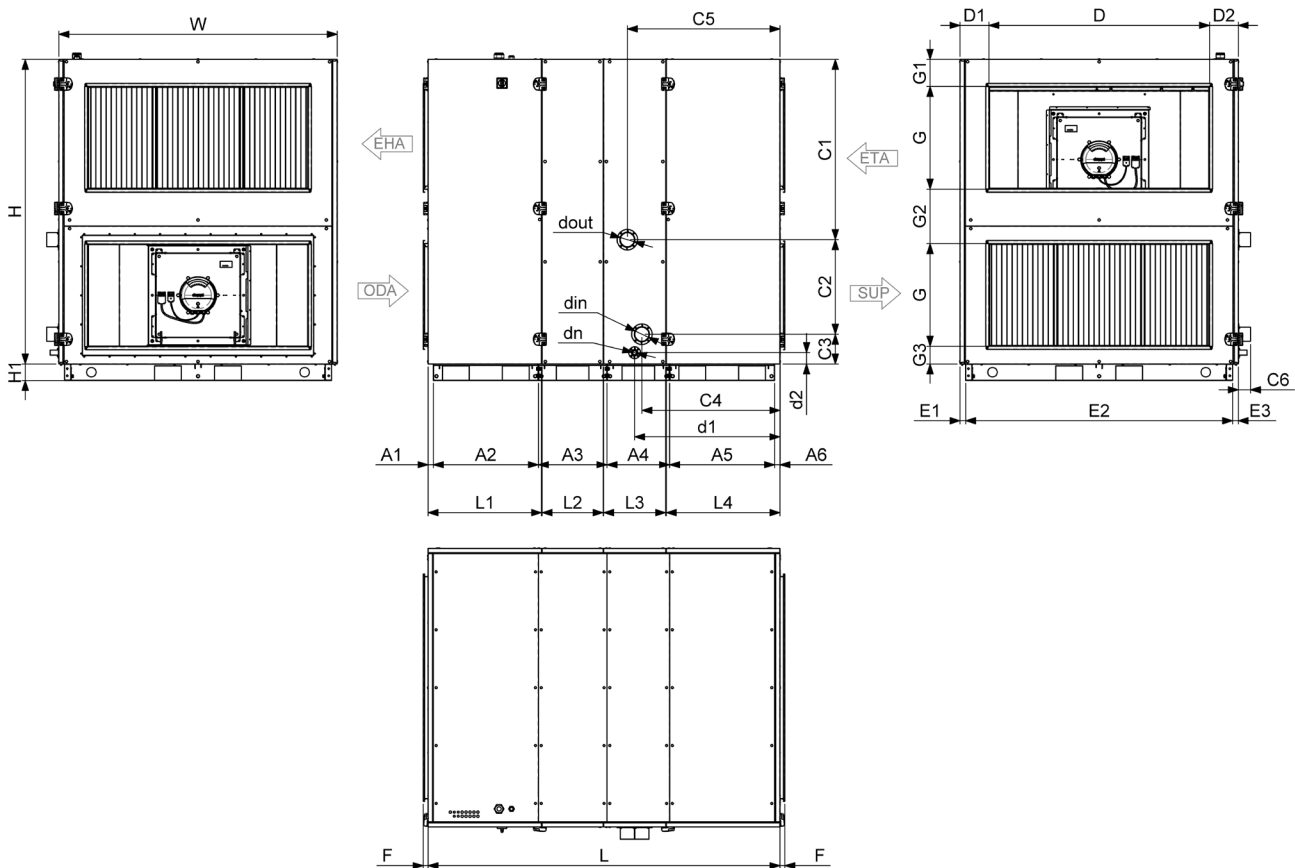
Fig. 8.1.24 Wymiary AmberAir Compact S-R-7000-H-CO-R-C1 / AmberAir Compact S-R-9000-H-CO-R-C1
