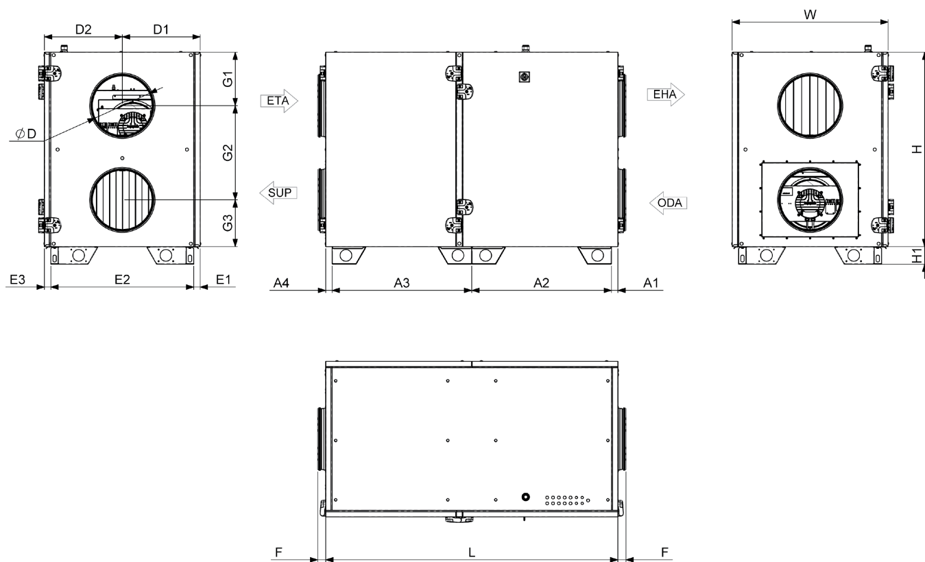
Fig. 8.1.1 Wymiary AmberAir Compact S-R-1000-H-E-L-C1 / AmberAir Compact S-R-1500-H-E-L-C1
