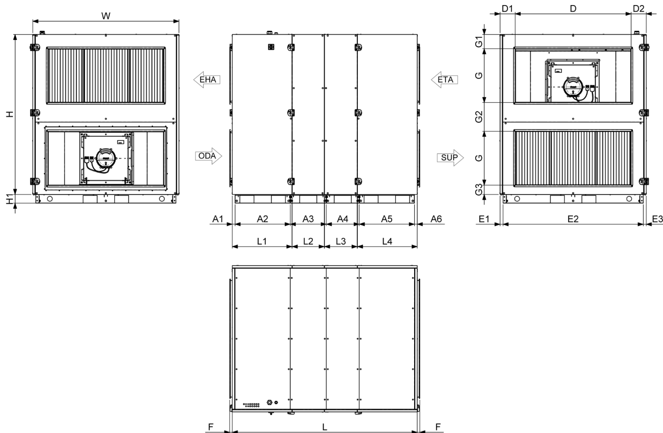
Fig. 8.1.22 Wymiary AmberAir Compact S-R-7000-H-E-R-C1 / AmberAir Compact S-R-9000-H-E-R-C1
