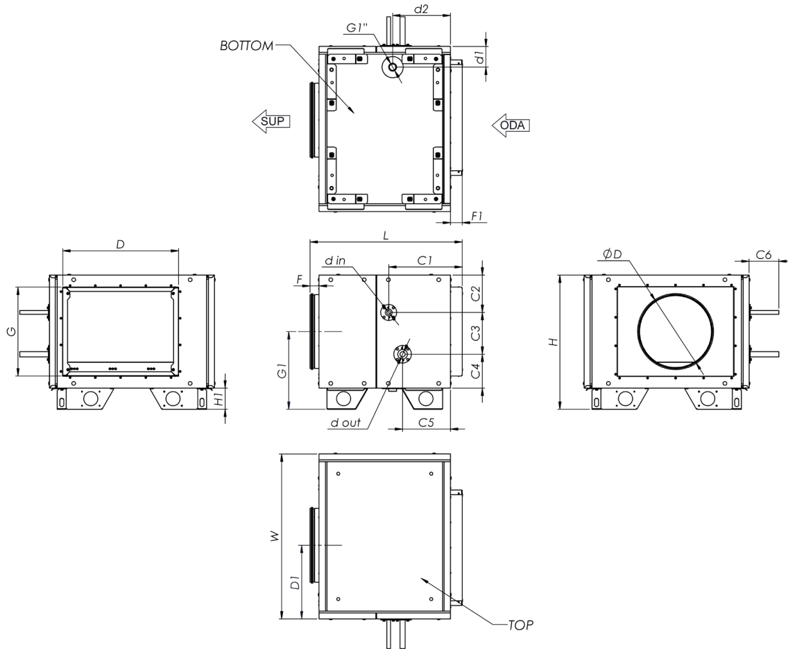
Fig. 8.1.34 Wymiary Comfort box DX left for AmberAir Compact-S-R-1000-H / AmberAir Compact S-R-1500-H / AmberAir Compact S-R-2000-H
