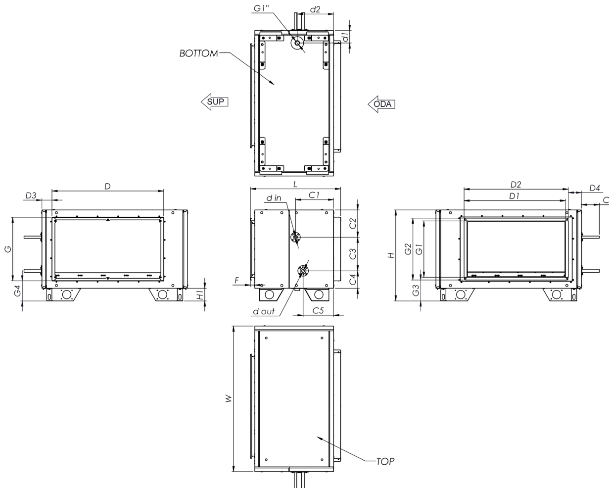
Fig. 8.1.35 Wymiary Comfort box DX left for AmberAir Compact S-R-3000-H
