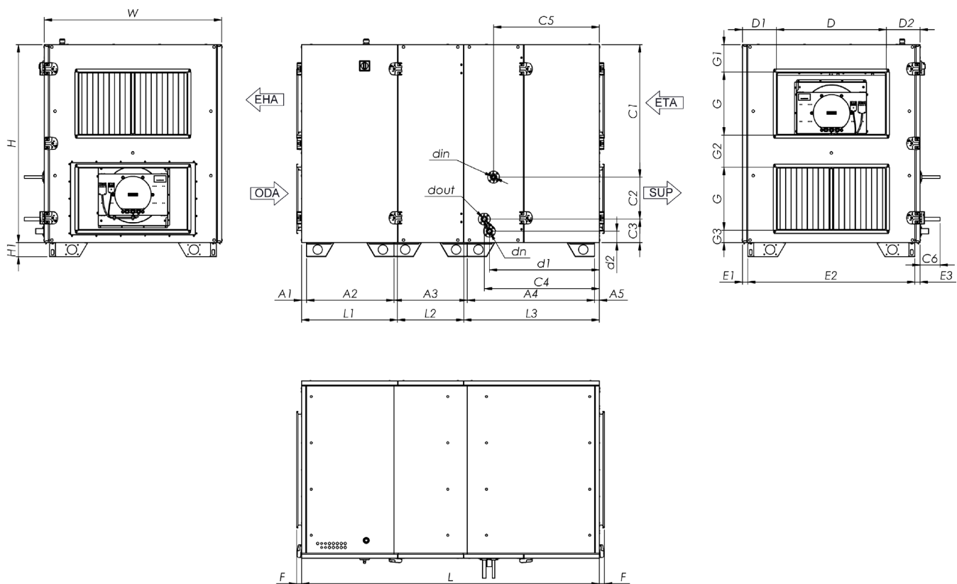
Fig. 8.1.18 Wymiary AmberAir Compact S-R-3000-H-DX-R-C1 / AmberAir Compact S-R-4000-H-DX-R-C1 / AmberAir Compact S-R-5000-H-DX-R-C1
