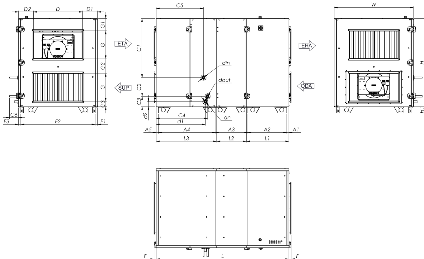
Fig. 8.1.17 Wymiary AmberAir Compact S-R-3000-H-DX-L-C1 / AmberAir Compact S-R-4000-H-DX-L-C1 / AmberAir Compact S-R-5000-H-DX-L-C1
