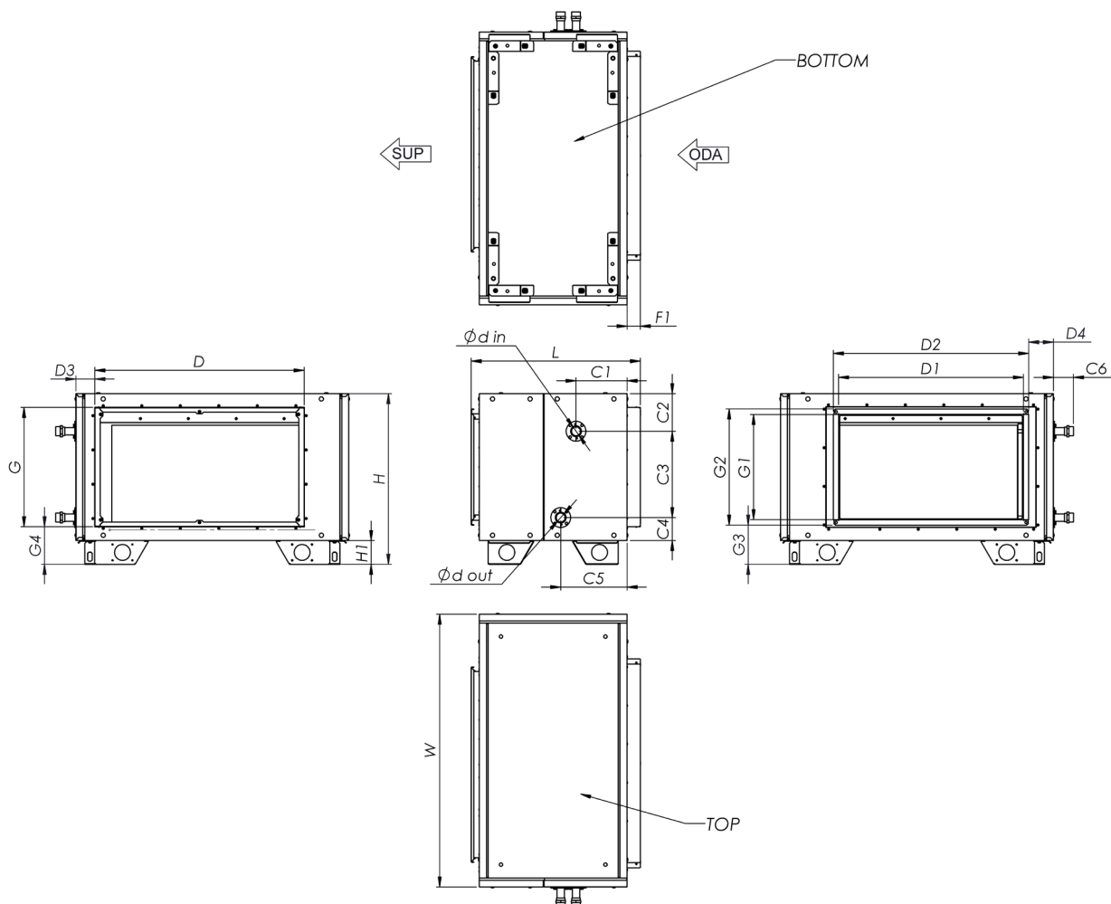
Fig. 8.1.33 Wymiary Comfort box WH left for AmberAir Compact S-R-3000-H
