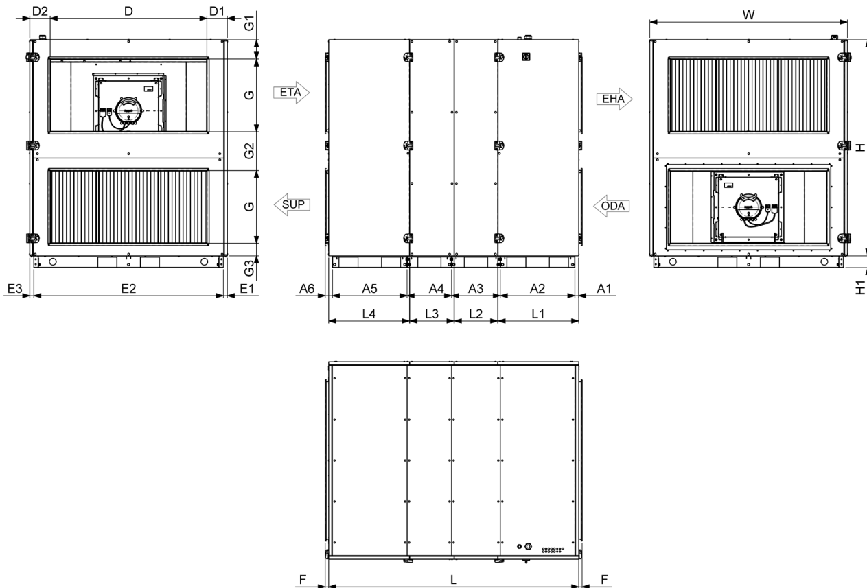
Fig. 8.1.21 Wymiary AmberAir Compact S-R-7000-H-E-L-C1 / AmberAir Compact S-R-9000-H-E-L-C1
