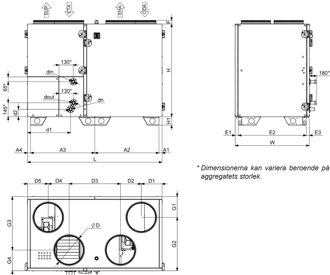
Fig. 8.1.5 AmberAir Compact S-R-1000-V-DX-L-C1 / AmberAir Compact S-R-1500-V-DX-L-C1 dimensioner
