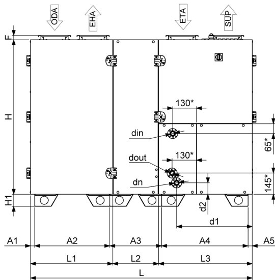
Fig. 8.1.11 AmberAir Compact-S-R-2000-V-DX-L-C1 / AmberAir Compact-S-R-3000-V-DX-L-C1 / AmberAir Compact-S-R-4000-V-DX-L-C1 / AmberAir Compact-S-R-5000-V-DX-L-C1 dimensioner
