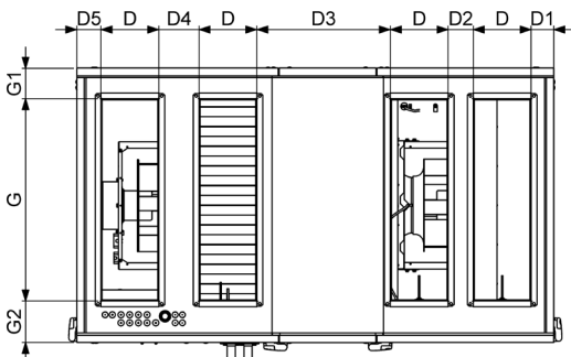
Fig. 8.1.11 AmberAir Compact-S-R-2000-V-DX-L-C1 / AmberAir Compact-S-R-3000-V-DX-L-C1 / AmberAir Compact-S-R-4000-V-DX-L-C1 / AmberAir Compact-S-R-5000-V-DX-L-C1 dimensioner
